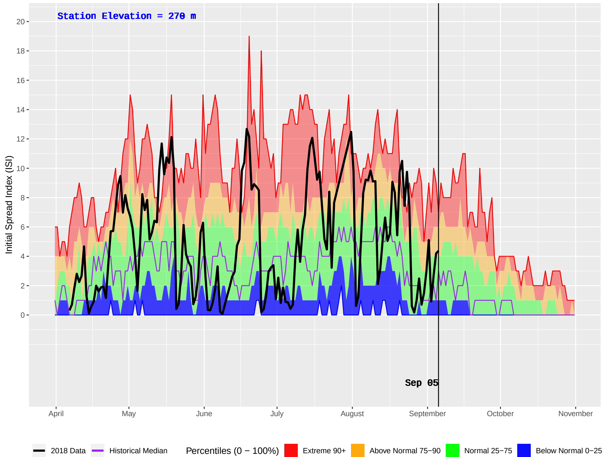
TALCHAKO (233) : Historical (1990–2016) and Current (2018) Daily Initial Spread Index (ISI)
